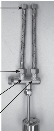
Anschluss 1/2" IG Connection 1/2" IG inside thread Anschluss 3/8" IG Connection 3/8" IG inside thread
