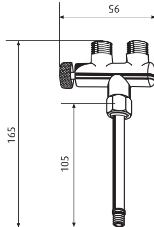
Ⓓ Abmessungen in mm Dimensions in mm
