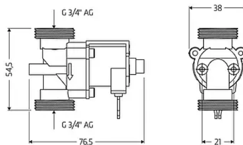
WimTec PROOF SV - Magnetventil:
